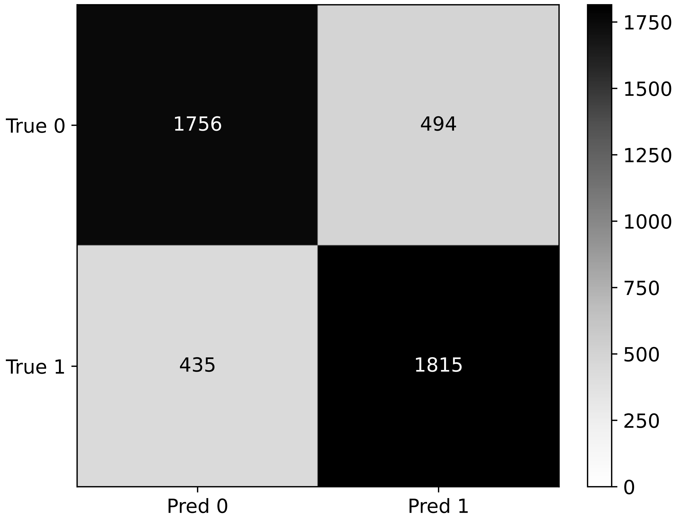
Confusion Matrix (test)
